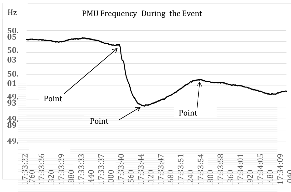
FIGURE A: SAMPLE PMU FREQUENCY PLOT SHOWING RELEVANT POINTS FOR FRC CALCULATION
