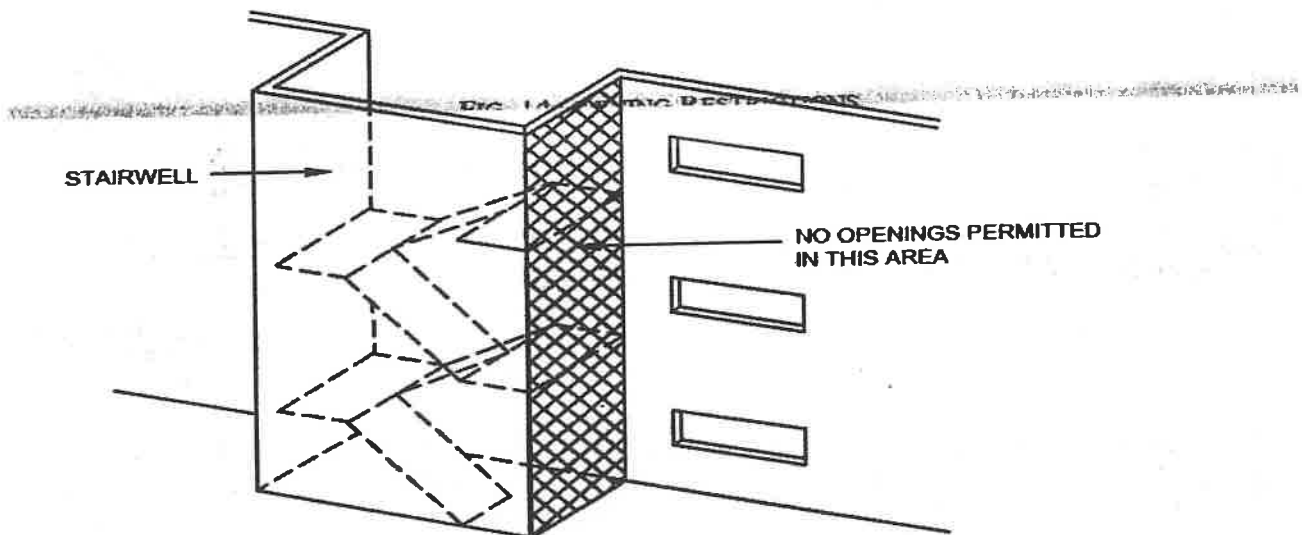
14B OPENING RESTRICTIONS ON STAIRWELL WALLS
