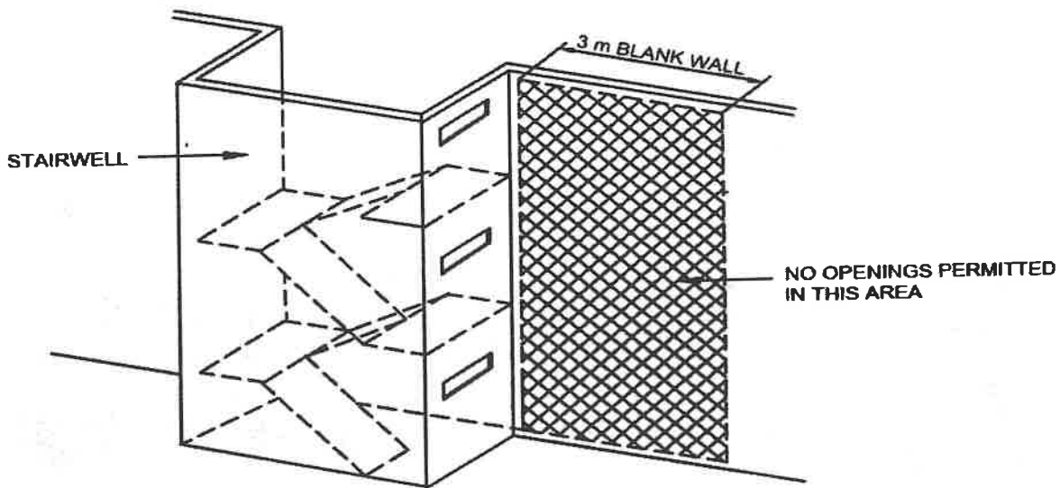
14A LIMITATIONS ON OPENINGS NEAR STAIRWELL
