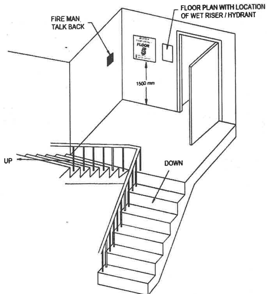
9B STAIR SIGN PLACEMENT
