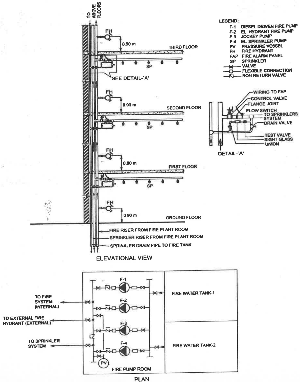
FIG. 16 TYPICAL SYSTEM OF PUMPING WITH TWO ELECTRIC, ONE DIESEL FIRE PUMP
