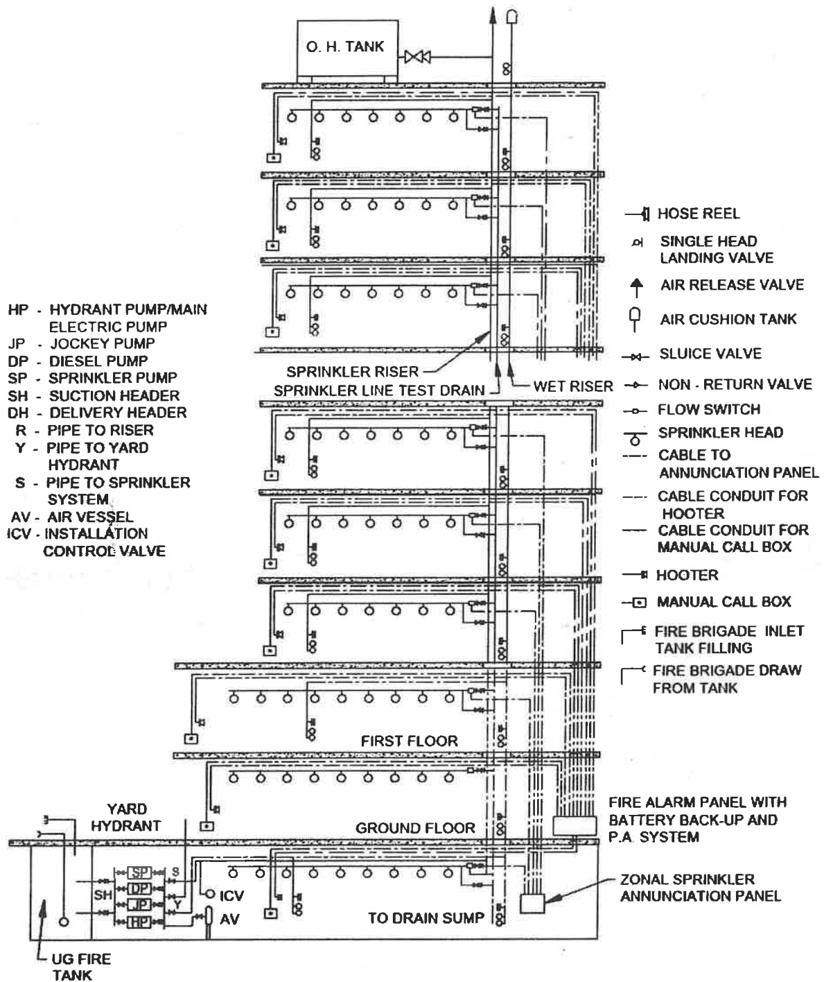
FIG. 17 TYPICAL ARRANGEMENT OF WET RISER AND TOTAL SPRINKLER SYSTEM OF BUILDING
