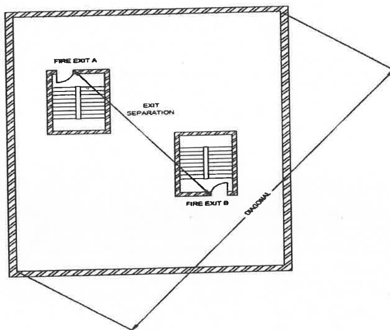
FIG. 10 FIRE EXIT SEPARATION
