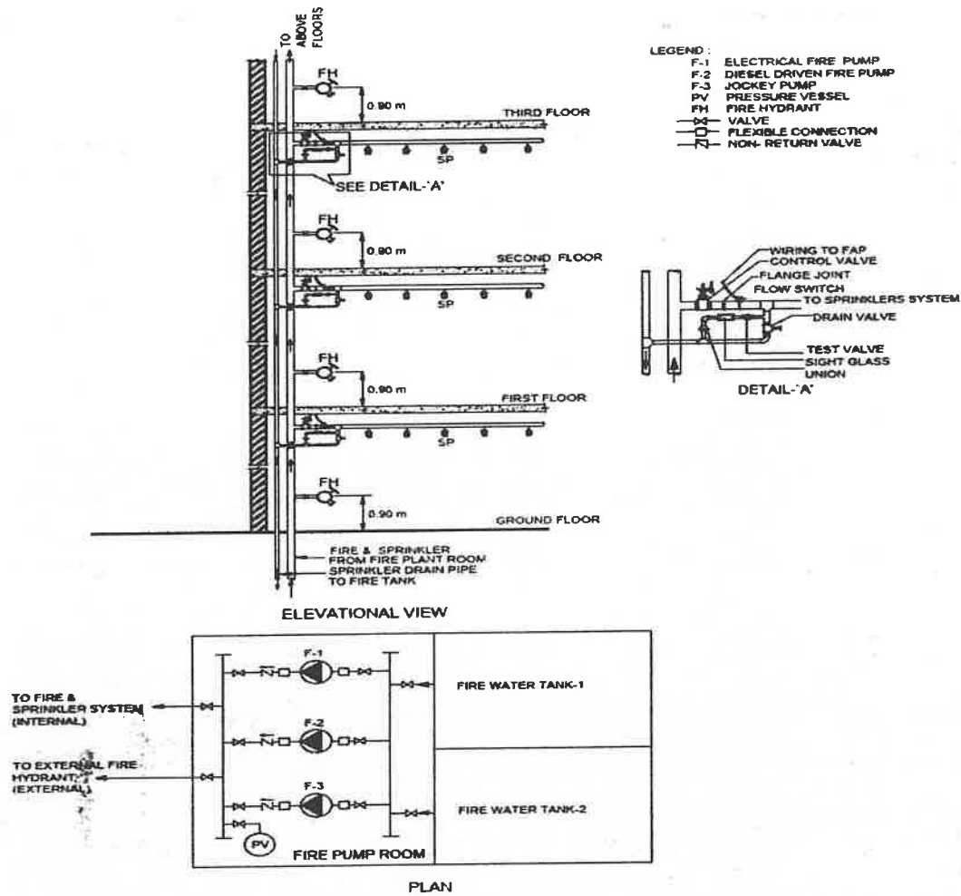
FIG. 15 TYPICAL SYSTEM OF PUMPING WITH ONE ELECTRIC, ONE DIESEL FIRE PUMP
