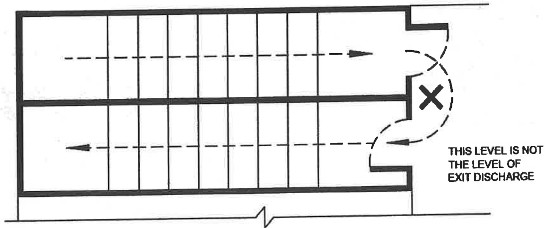
FIG. 11 UNACCEPTABLE ARRANGEMENT FOR ENCLOSING A STAIR SERVING AS A REQUIRED EXIT
