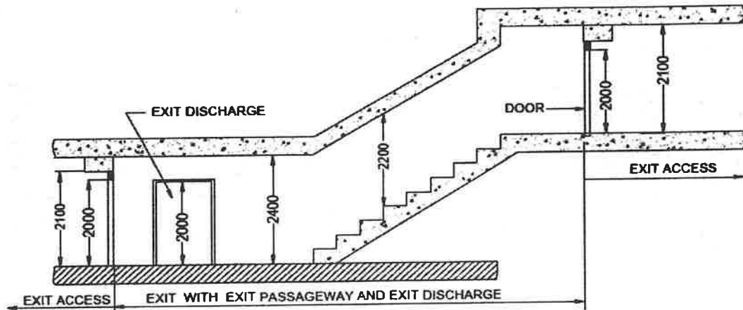
FIG. 8 MINIMUM HEAD ROOM MEASUREMENT
