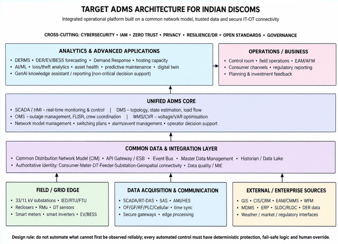
Figure 3A. Recommended target ADMS architecture for Indian DISCOMs.
